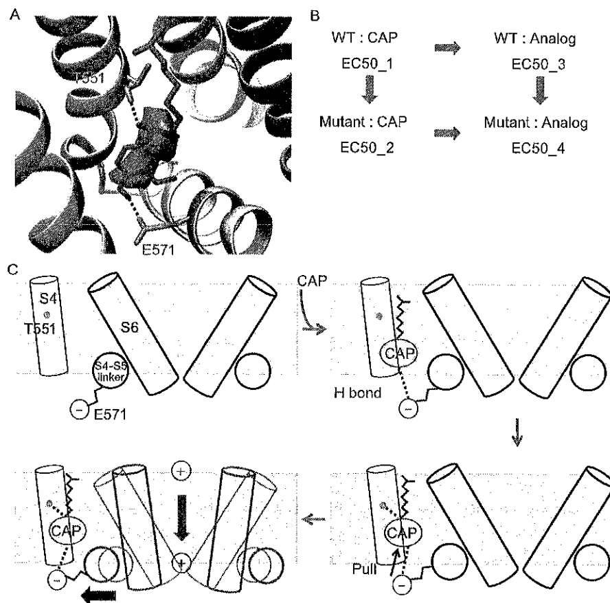
Figure 2. Mechanism of TRPV1 activation by capsaicin. (A) Docking of capsaicin into its binding pocket on open-state TRPV1 structure (PDB ID: 3J5R). The Head, Neck and Tail of capsaicin are colored in red, blue and magenta, respectively. Two residues making hydrogen bonds with capsaicin are highlighted in orange. Note that the amino acid numbering for mouse TRPV1 differs from that for rat and human TRPV1 (Fig. 1) by one. (B) Diagram showing the principle of thermodynamic mutant cycle analysis. (C) Cartoon summarizing capsaicin binding and activation of TRPV1.
